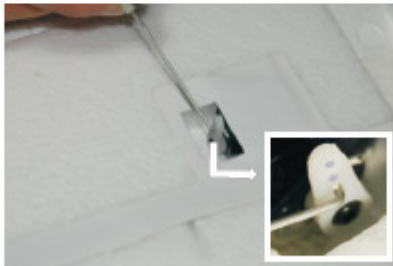
15. Install the linkage rod of the flap inside the lowest hole of the servo horn.
